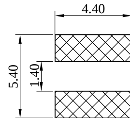
( PCB Pattern )
